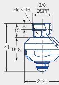
Compact version Male thread
